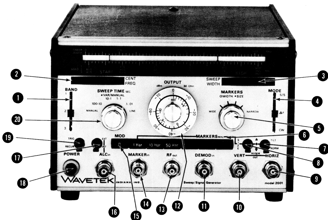
Figure 3-1. Front Panel
