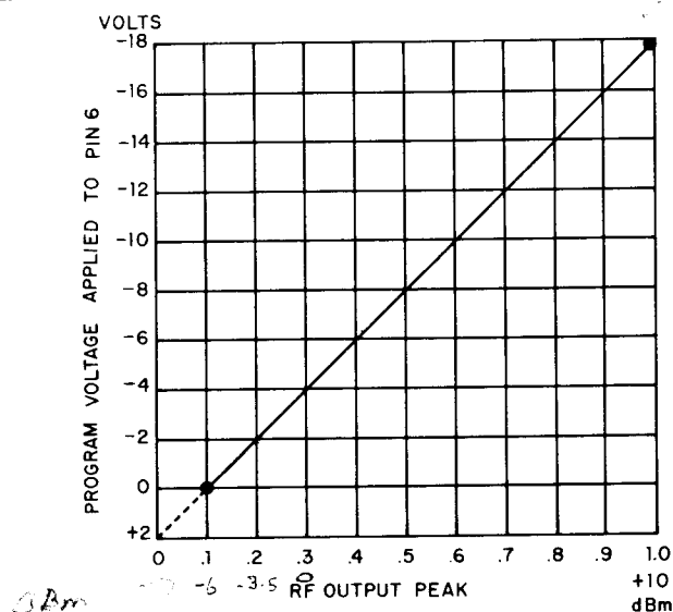
Figure 3-6. Program Voltage/Rf Output
