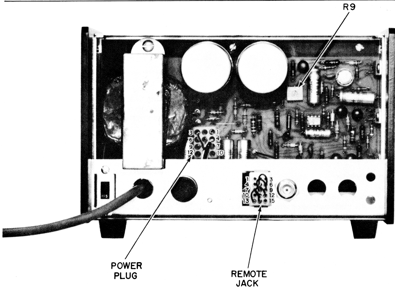
Figure 5-8. Power Supply
