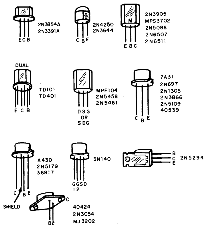
Figure 5-3. Transistor Lead Configuration
